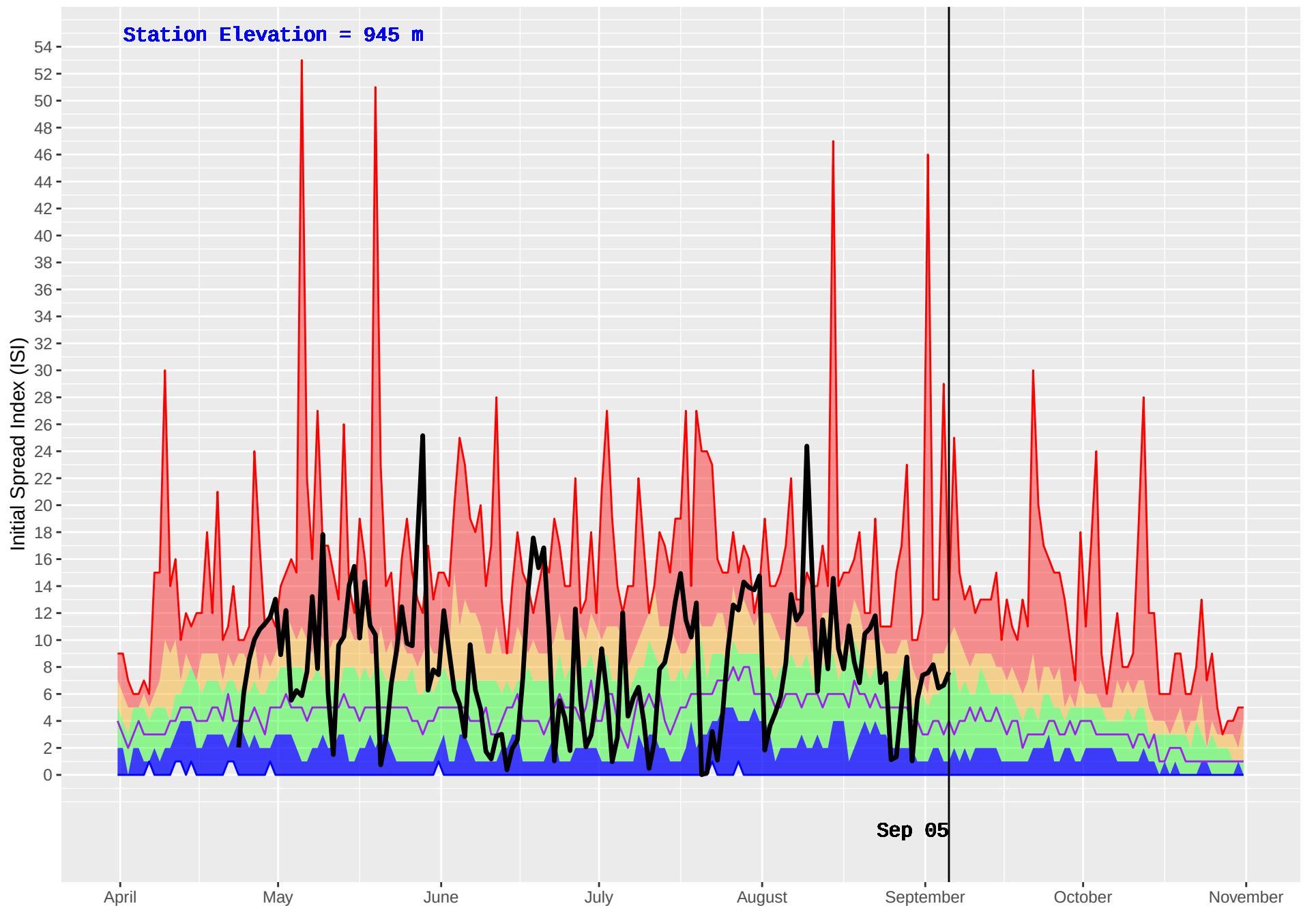
TATLA LAKE HUB (208) : Historical (1980–2016) and Current (2018) Daily Initial Spread Index (ISI)
