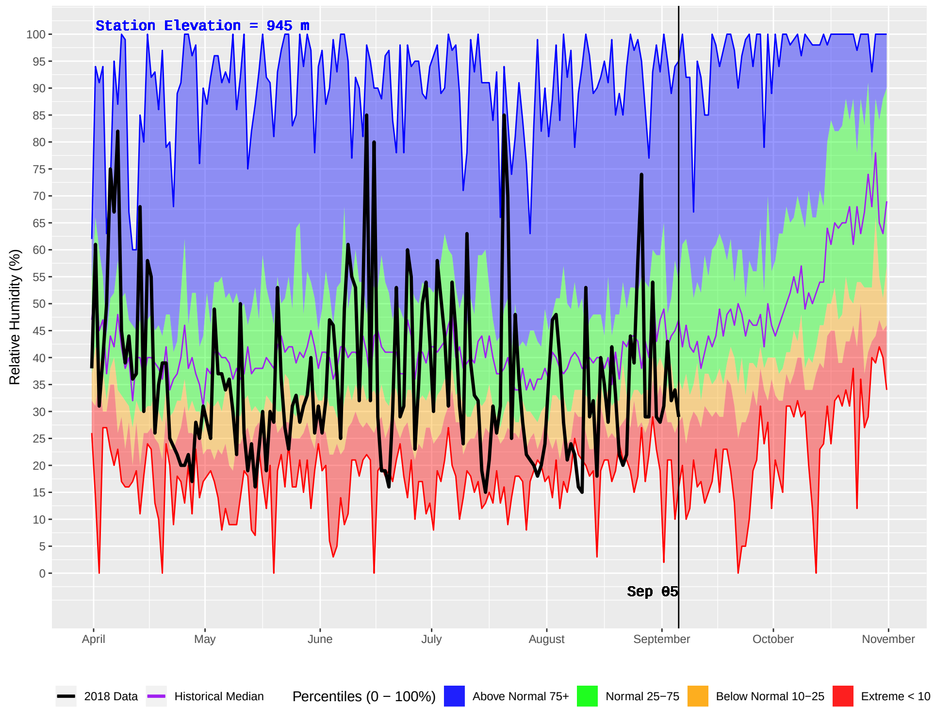
TATLA LAKE HUB (208) : Historical (1980–2016) and Current (2018) Daily Relative Humidity
