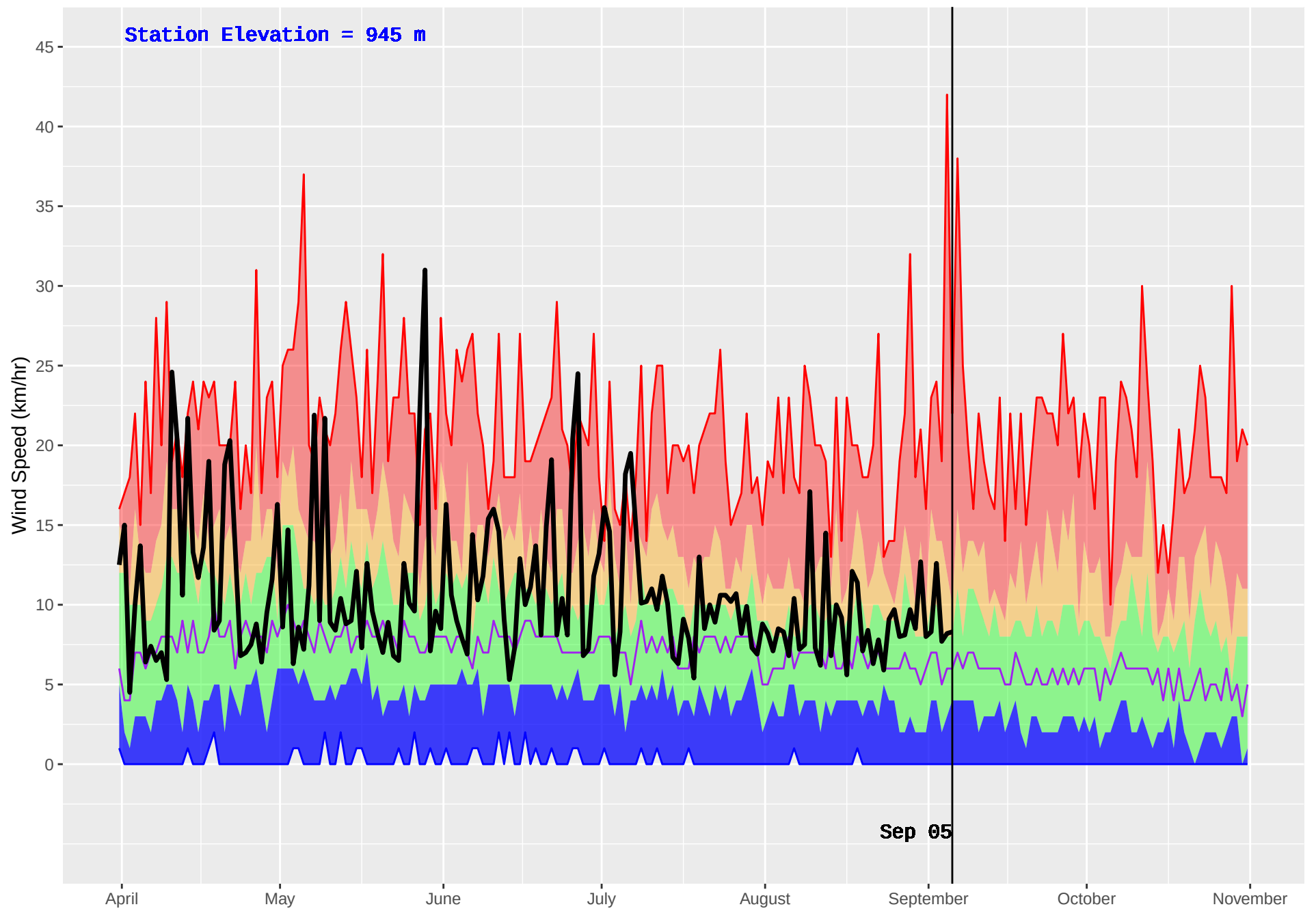
TATLA LAKE HUB (208) : Historical (1980–2016) and Current (2018) Daily Wind Speed
