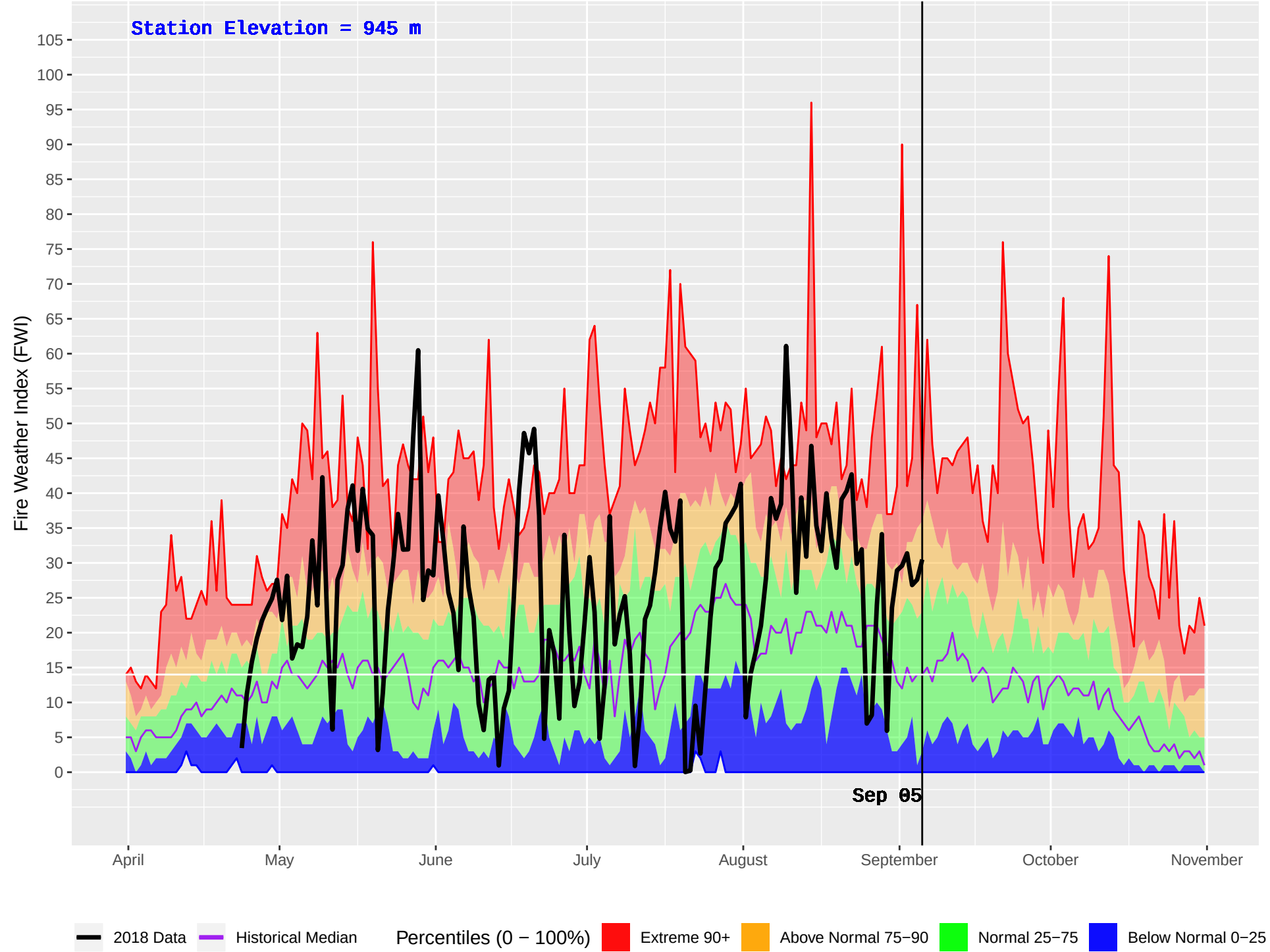
TATLA LAKE HUB (208) : Historical (1980–2016) and Current (2018) Daily Fire Weather Index (FWI)
