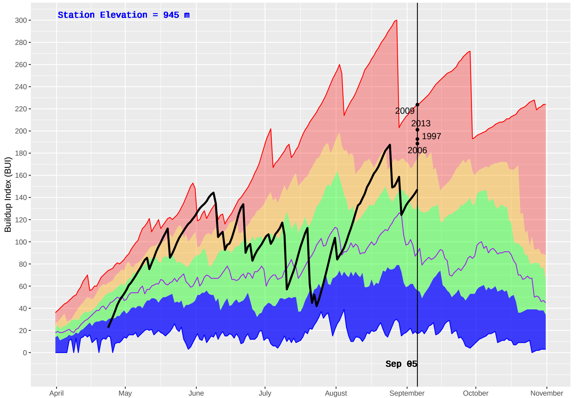
TATLA LAKE HUB (208) : Historical (1980–2016) and Current (2018) Daily Buildup Index (BUI)
