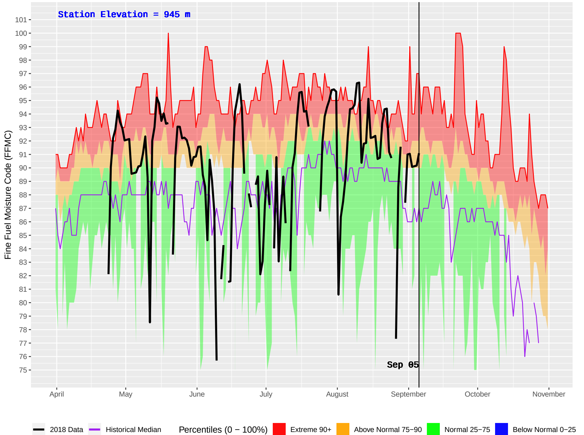
TATLA LAKE HUB (208) : Historical (1980–2016) and Current (2018) Daily Fine Fuel Moisture Code (FFMC)
